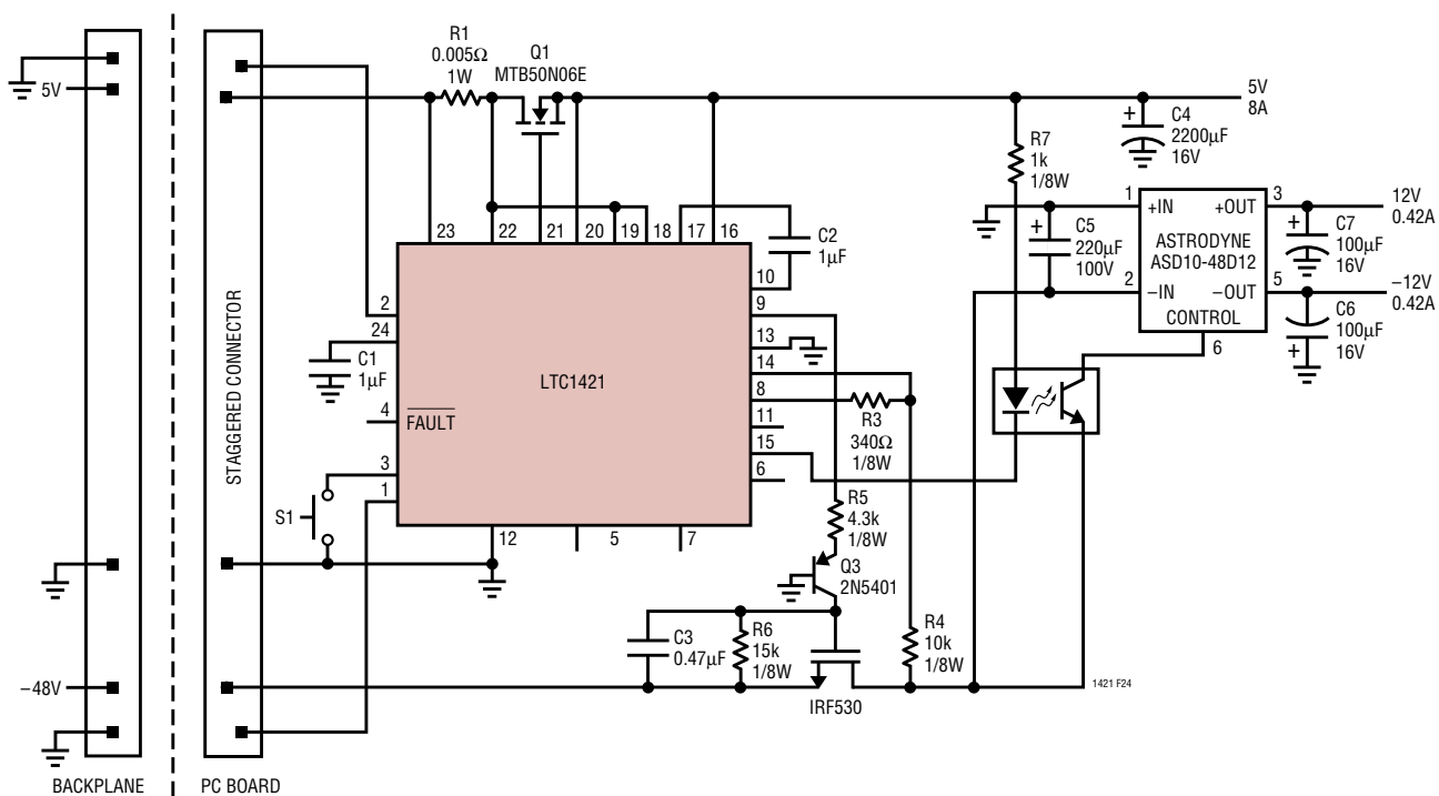
Figure 24. 5V and -48V to \pm 12\text{V} Hot Swappable Supply
