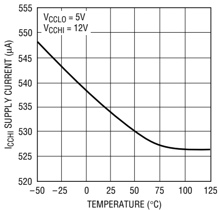
ICCI Supply Current vs Temperature
