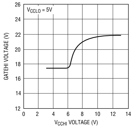
GATEHI Voltage vs VCCI Voltage
