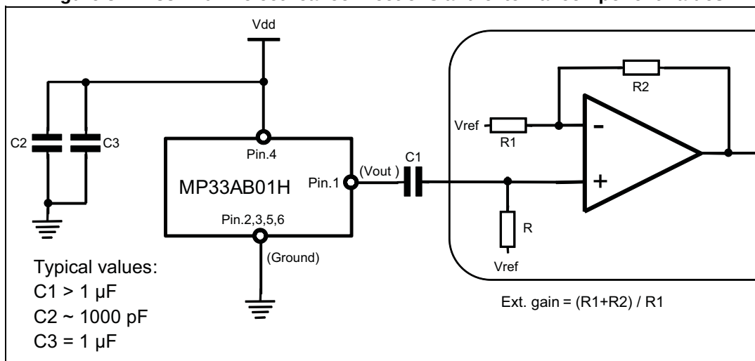
Figure 3. MP33AB01H electrical connections and external component values
