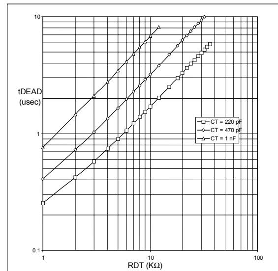
Figure 27: Deadtime vs R_{DT}
