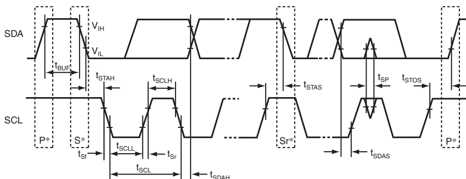
Figure 20.3 Input Timing
