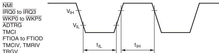
Figure 20.3 Input Timing
