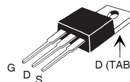
TO-3P (IXTQ)
