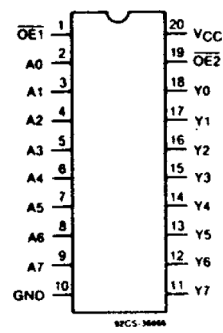
Figure 3-2. CDx4AC541, CDx4ACT541
