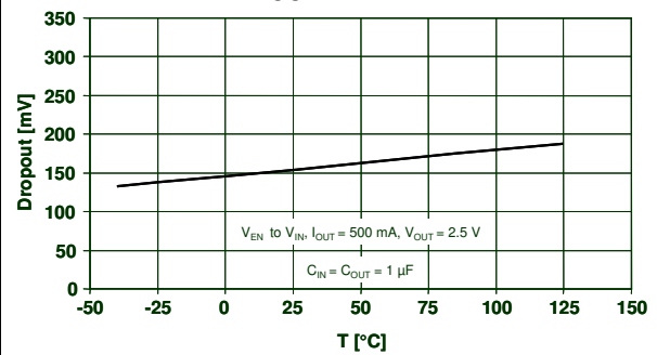
Figure 8. Dropout voltage vs. temperature ( V_{OUT} = 2.5 V)
