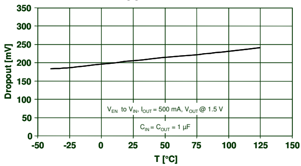
Figure 7. Dropout voltage vs. temperature ( V_{OUT} = 1.5 V)
