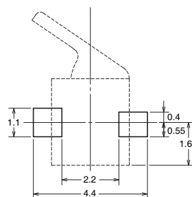
PCB land dimensions (reference) (TOP VIEW)
