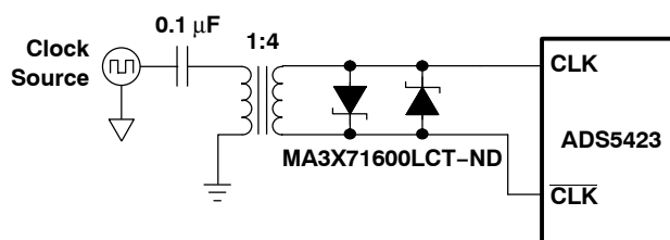
Figure 42. Differential Clock
