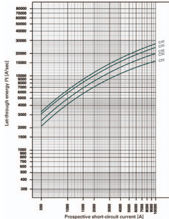
Characteristic C (40A), 240V
