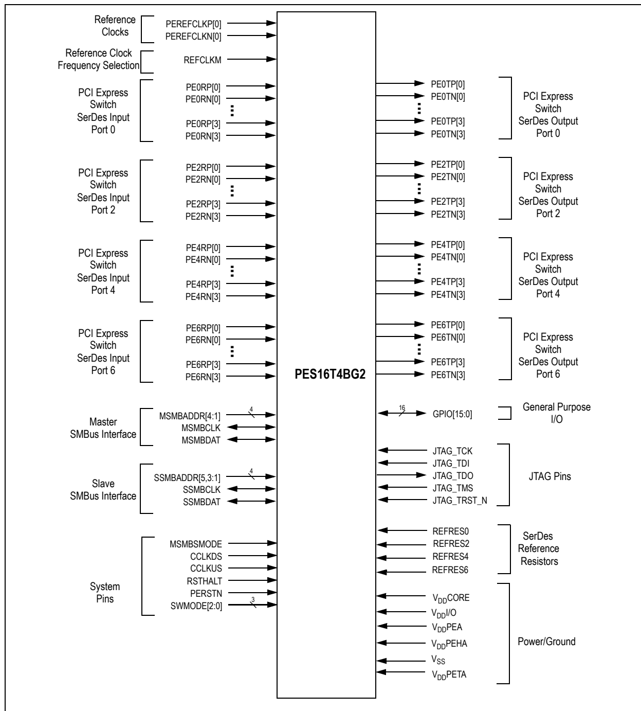
Figure 4 PES16T4BG2 Logic Diagram
