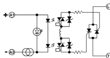
DC Input Equivalent Circuit
