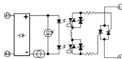
AC Input Equivalent Circuit
