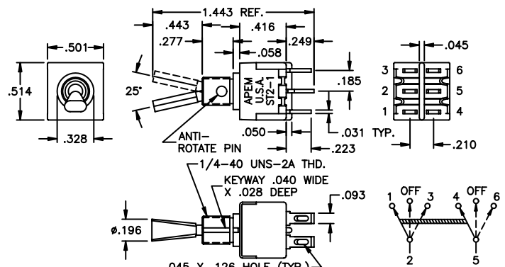
DOUBLE POLE
