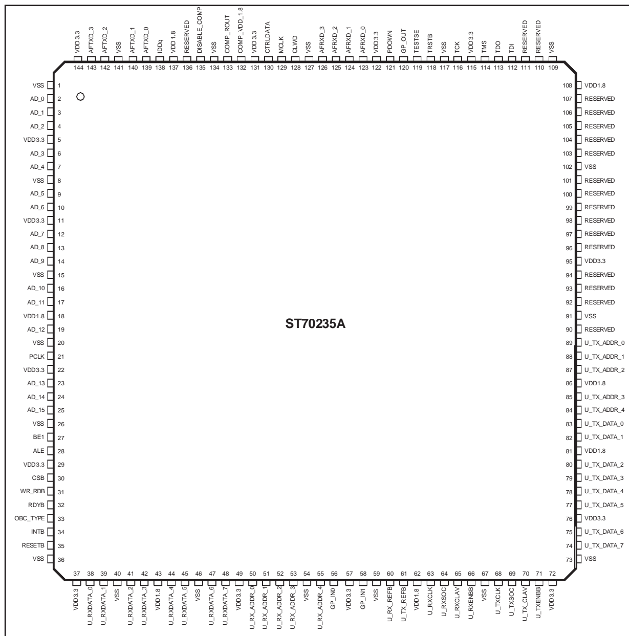
Figure 2 : Pin Connection
