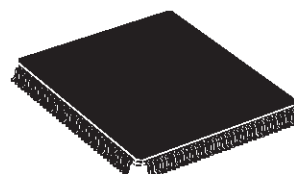
TQFP144 Full Plastic (20 x 20 x 1.40 mm)
