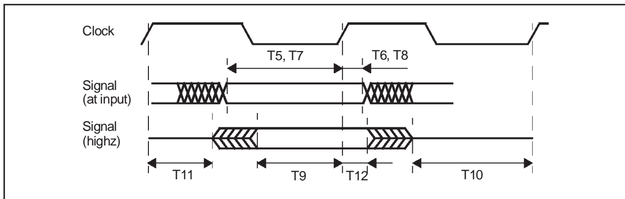
Figure 16 : Timing Specification (Utopia 2)
