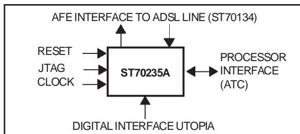
Figure 9 : ST70235A Interfaces
