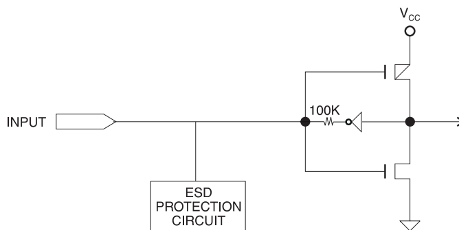
Figure 8-1. Input Diagram
