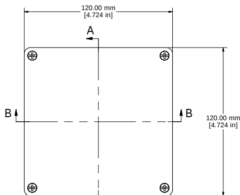
ASSEMBLY
