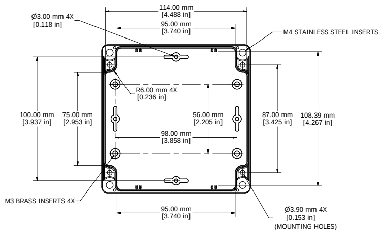
BOX - INSIDE
