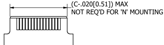
PCB LAYOUT RECOMMENDED (FOR __B__DYRN, __B__DYRD OR __B__DYRT)
