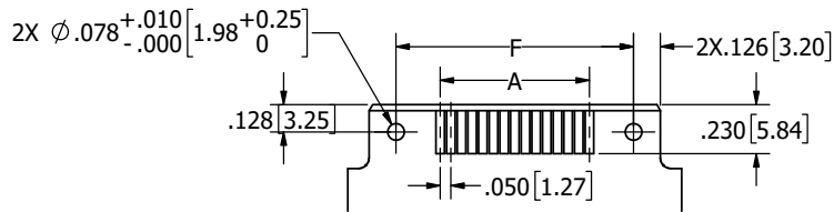
PCB LAYOUT RECOMMENDED (FOR __B__DYRQ)
