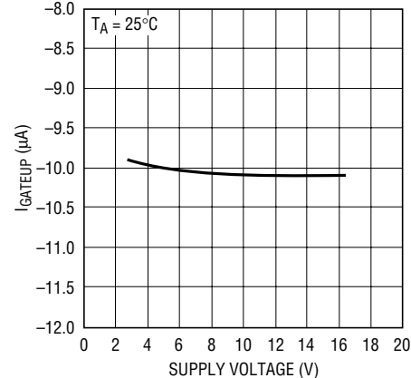
I_{\text{GATEUP}} vs Supply Voltage
