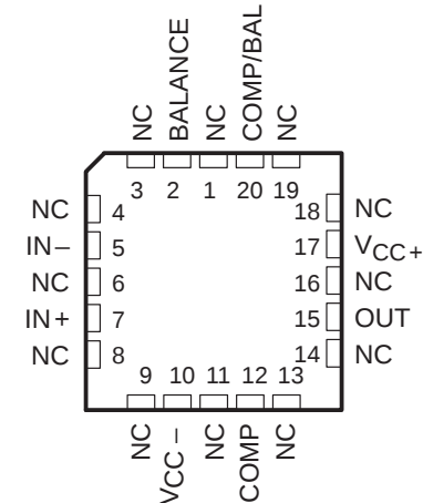
SE5534, SE5534A . . . FK PACKAGE (TOP VIEW)
