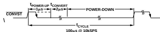
Figure 11. Automatic Power-Down
