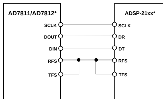
Figure 24. Interfacing to the ADSP-21xx
