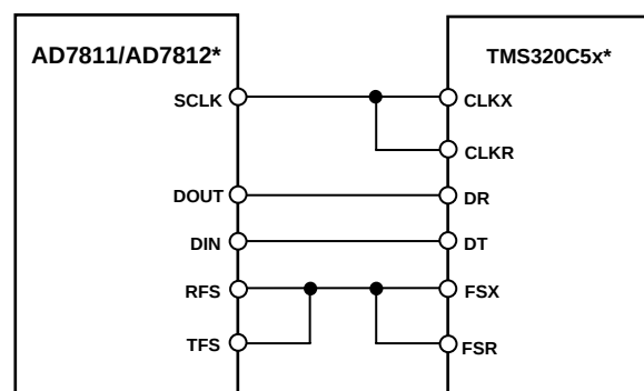
Figure 23. Interfacing to the TMS320C5x
