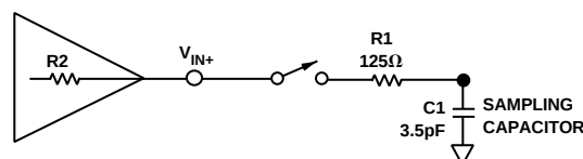
Figure 8. Equivalent Sampling Circuit
