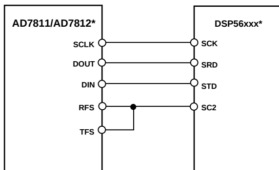
Figure 25. Interfacing to the DSP56xxx
