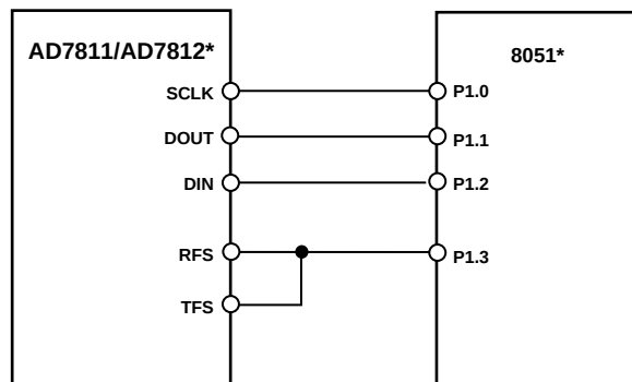
Figure 22. Interfacing to the 8051 Using I/O Ports
