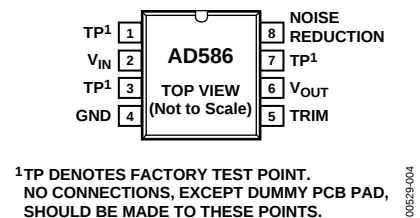
Figure 4. Pin Configuration (R-8)
