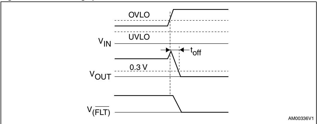
Figure 6. Overvoltage protection
