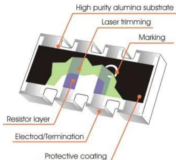
Fig 1. Constuction of a Chip-R array WA06X, 5% product
