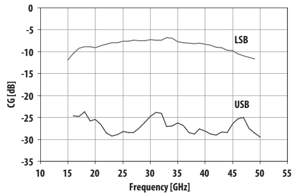
Figure 4. Typical conversion Gain, P_{lo}=+10\text{dBm} , IF_2=1\text{GHz}
