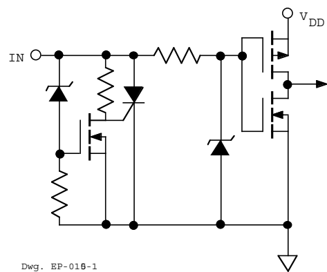
LOGIC INPUTS
