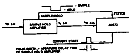
Figure 8. Sample-and-Hold Amplifier - AD572 Interconnections
