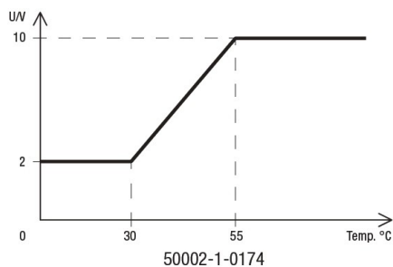
Control function: Both designs operate in cooling mode
