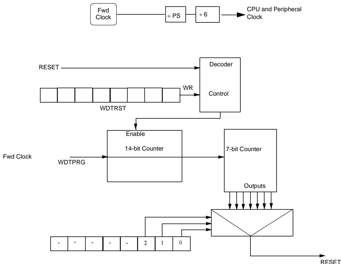
Figure 31. Watchdog Timer
