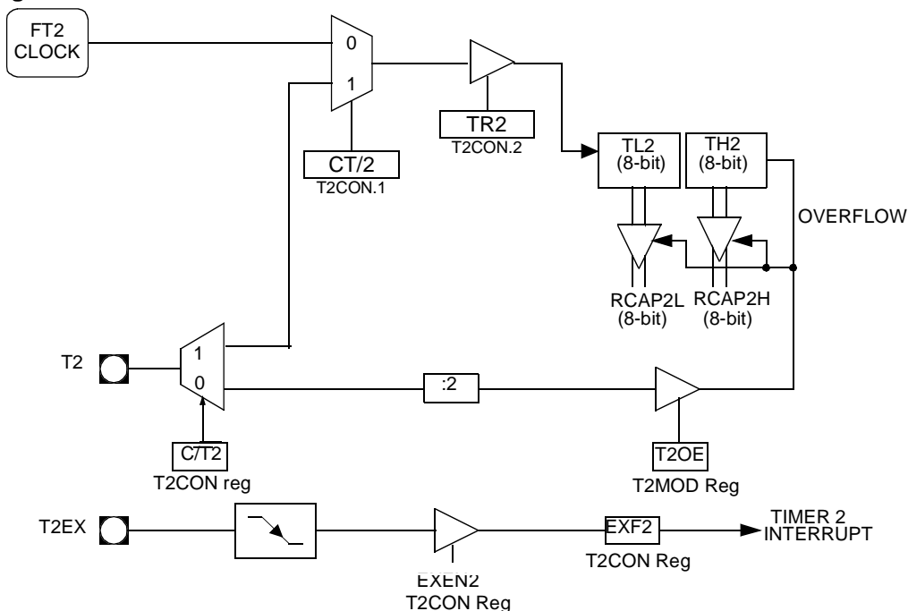
Figure 30. Clock-Out Mode
