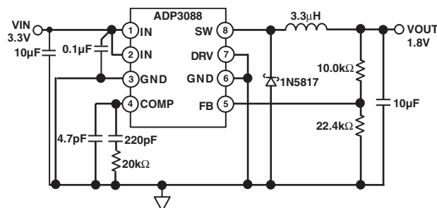
Figure 1. Typical Application
