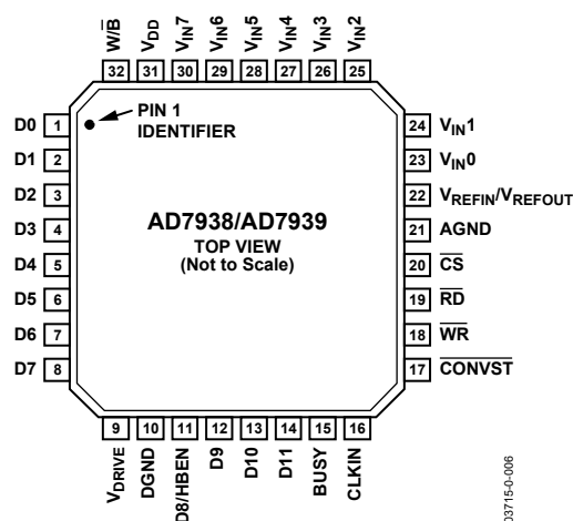
Figure 2. Pin Configuration
