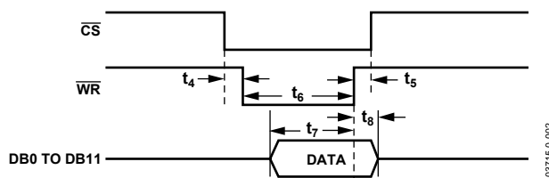
Figure 40. AD7938/AD7939 Parallel Interface—Write Cycle Timing for Word Mode Operation ( \overline{W/\overline{B}} = 1 )
