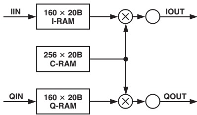
Figure 30. RAM Coefficient Filter (RCF) Block Diagram
