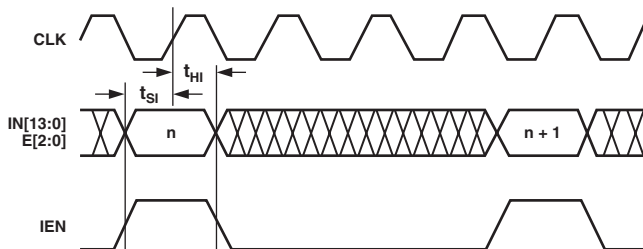
Figure 29. Fractional Rate Input Timing (4 × CLK) in Mode 01
