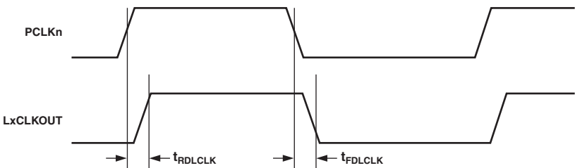
Figure 17. LxCLKOUT to PCLKn ( n = 0 and x = A, B ; or n = 1 and x = C, D ) Switching Characteristics
