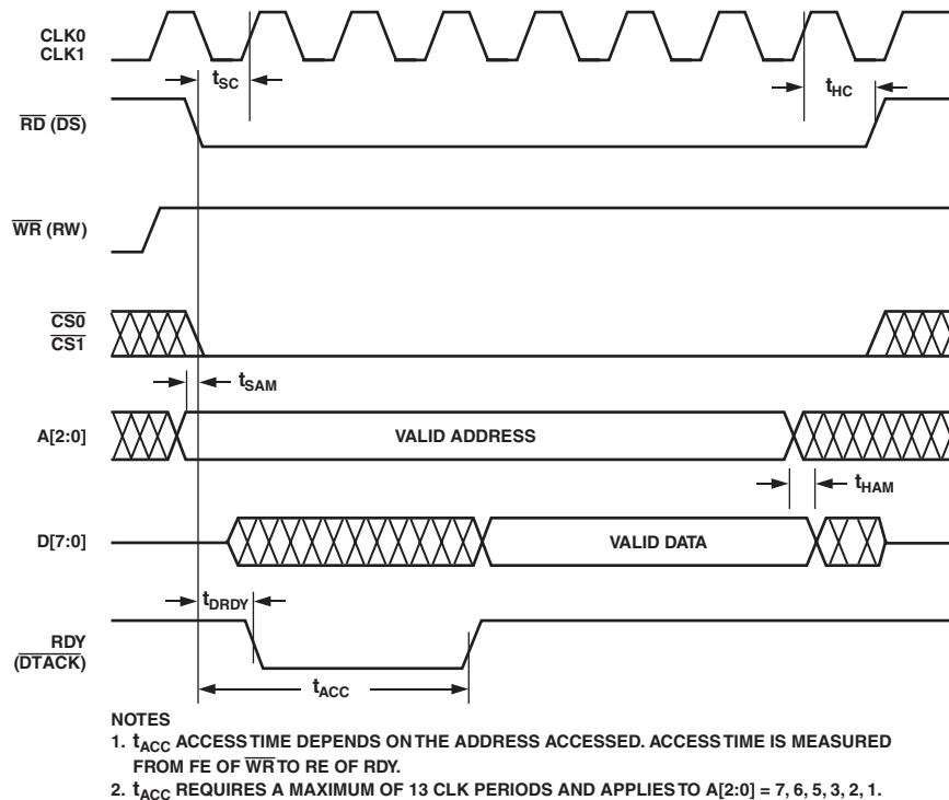
Figure 21. INM Microport Read Timing Requirements. CLK0 corresponds to \overline{CS0} , and CLK1 to \overline{CS1} . \overline{CS0} and \overline{CS1} both active (low) at the same time will cause contention on data bus.
