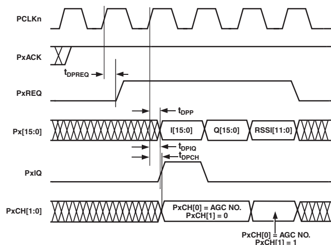
Figure 38. AGC with RSSI Word
