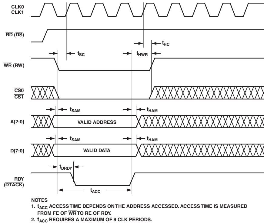
Figure 20. INM Microport Write Timing Requirements. CLK0 corresponds to \overline{CS0} , and CLK1 to \overline{CS1} . \overline{CS0} and \overline{CS1} both active (low) at the same time will cause errors in writing.
