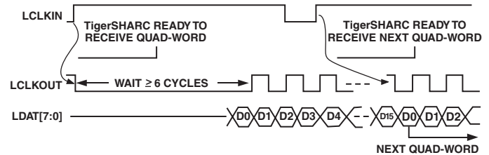
Figure 42. Link Port Data Transfer
