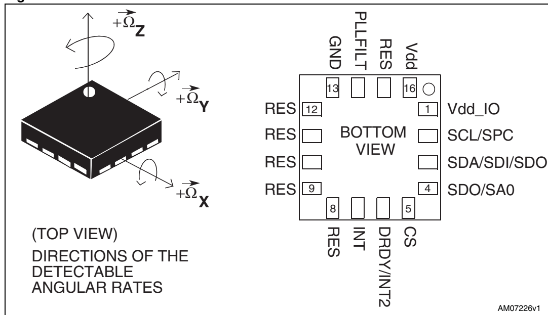
Figure 2. Pin connection
