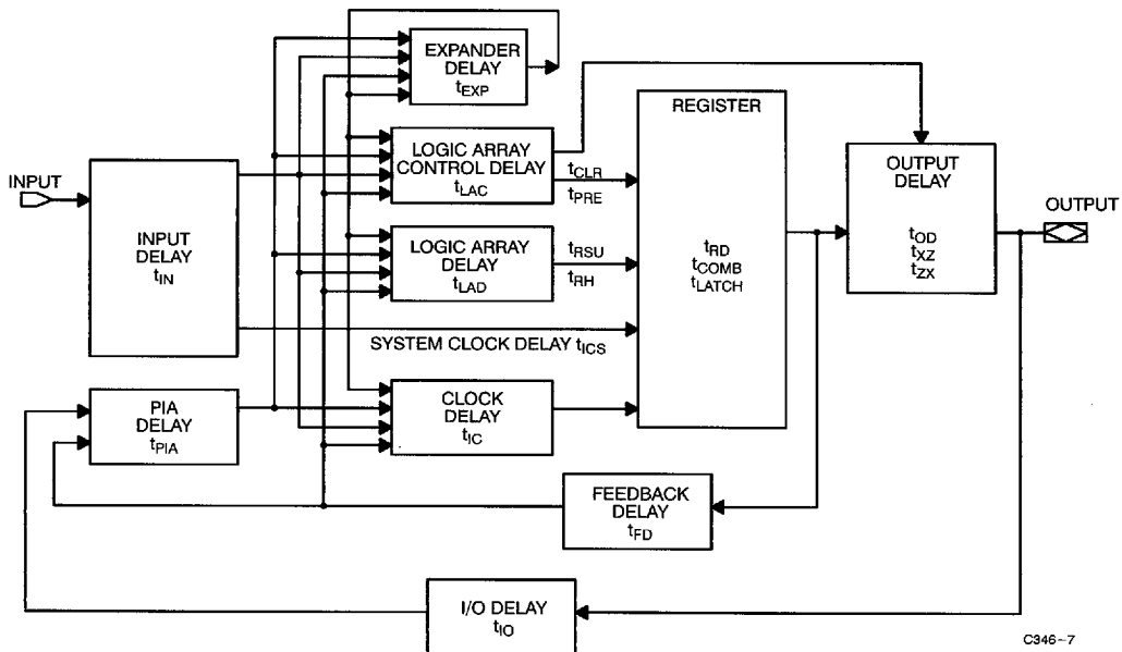
Figure 1. CY7C346/CY7C346B Internal Timing Model
