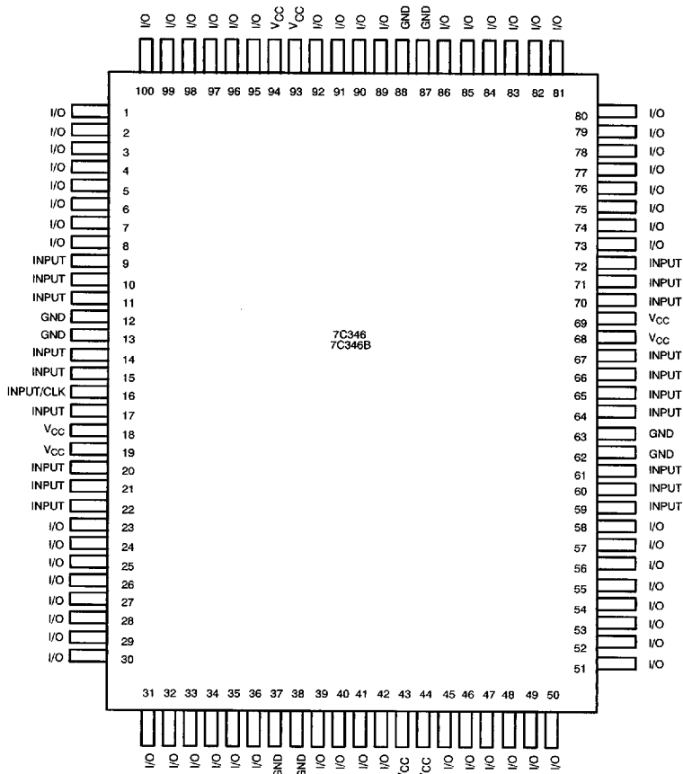
PQFP Top View
