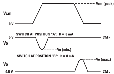
Figure 17. Test circuit for common mode transient immunity and typical waveforms.
