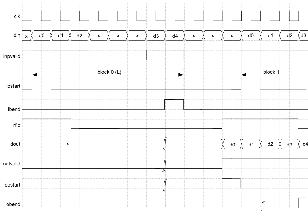
Figure 2-10. Timing Diagram for a Rate 1/2 Block Non-punctured Encoder with Tail Adding Inside
