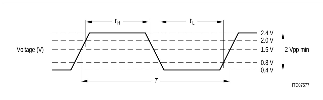
Figure 5-6 PCI Clock Specification
