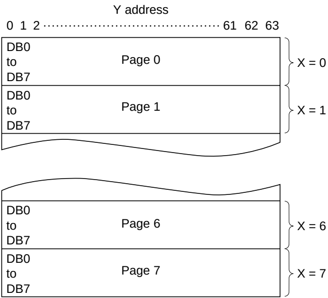
Figure 5 Address Configuration of Display Data RAM
