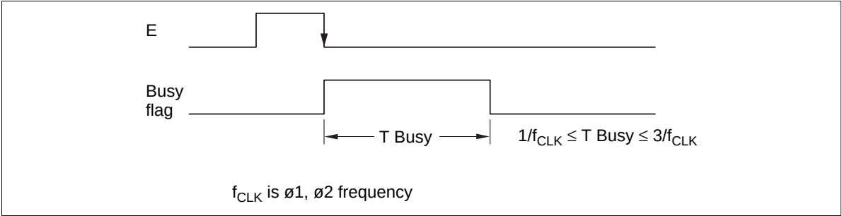
Figure 2 Busy Flag
