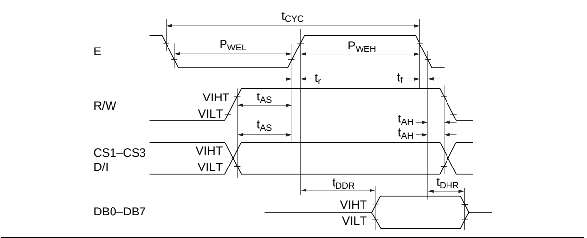
Figure 10 MPU Read Timing
