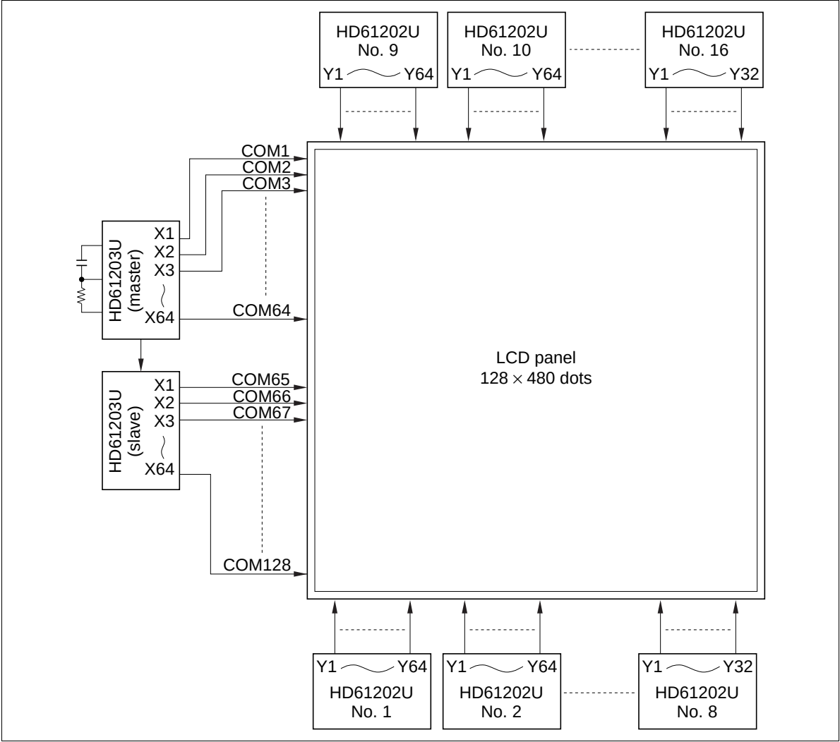
Figure 8 Application Example
