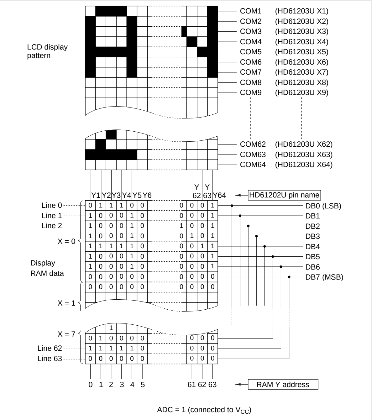
Figure 3 Relation between RAM Data and Display
