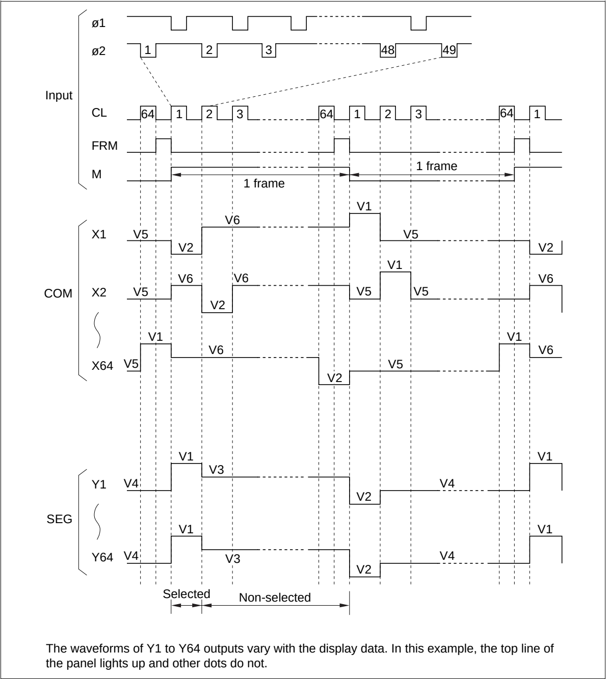
Figure 6 LCD Driver Timing Chart (1/64 Duty Cycle)
