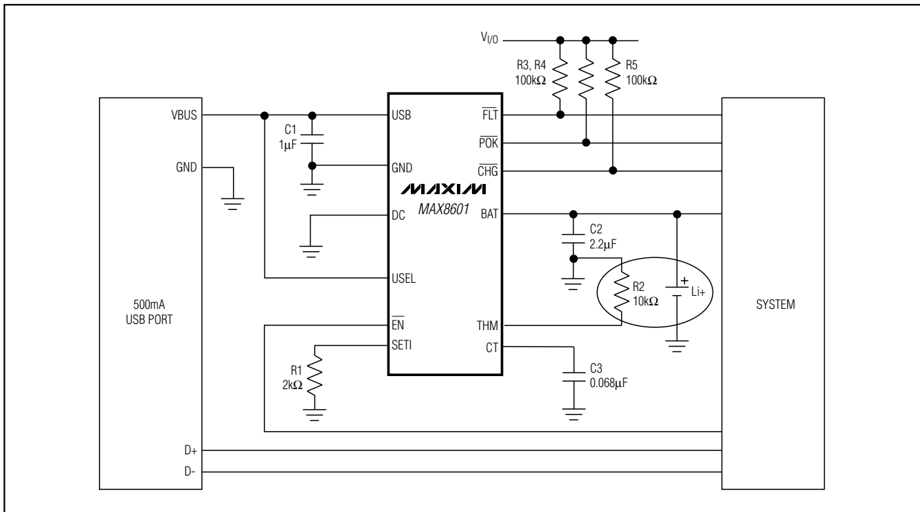
Figure 4. USB Battery Li Charger with the MAX8601
