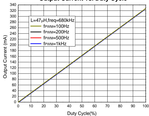
PWM Dimming ( V_{IN}=16\text{V} , 3LEDs, 47\mu\text{H} , R_s=0.3\Omega ) Output Current vs. Duty Cycle
