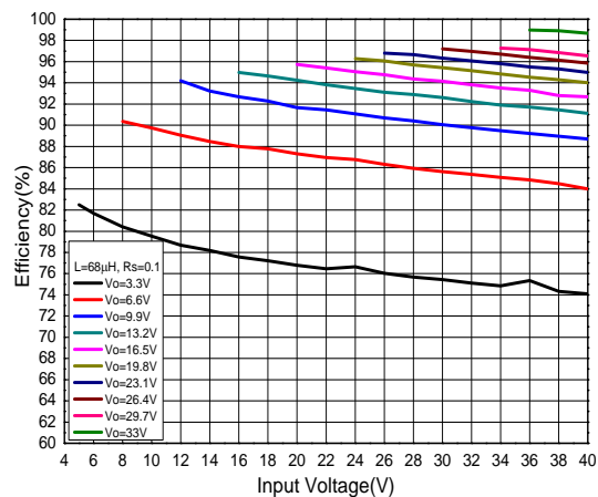
Efficiency vs. Input Voltage (MSOP-8EP, R s =0.1Ω, L=68μH)
