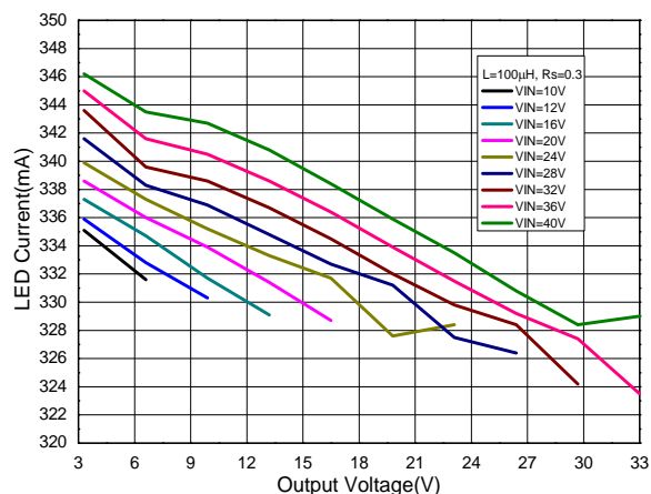
LED Current vs. Output Voltage (TSOT25, R s = 0.3Ω, L = 100μH)
