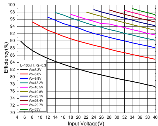
Efficiency vs. Input Voltage (TSOT25, R s =0.3Ω, L=100μH)
