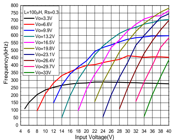
Operating Frequency vs. Input Voltage (TSOT25, R s =0.3Ω, L=100μH)
