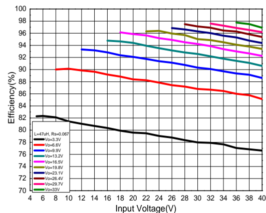
Efficiency vs. Input Voltage (MSOP-8EP, R s =0.067Ω, L=47μH)
