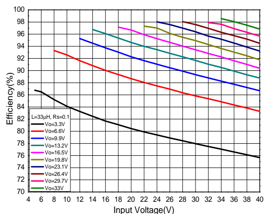
Efficiency vs. Input Voltage (TSOT25, R s =0.1Ω, L=33μH)
