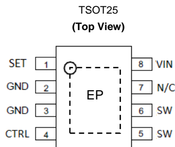
MSOP-8EP
