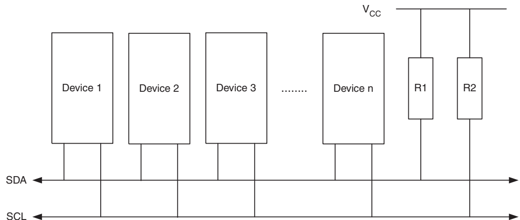
Figure 18-1. Two-Wire Bus Configuration
