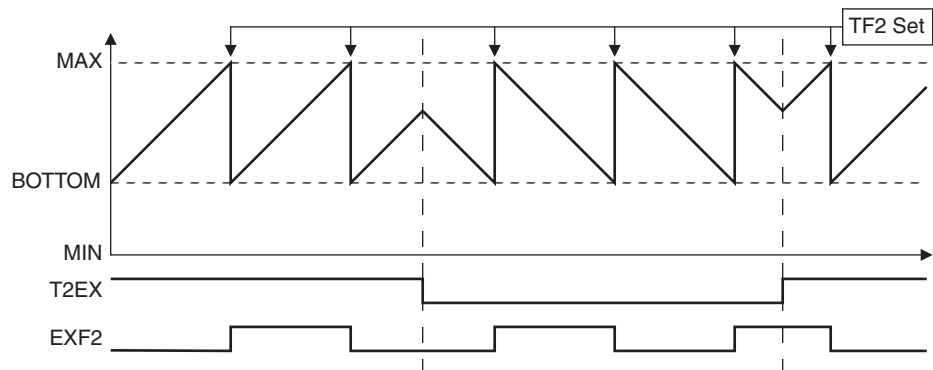
Figure 13-4. Timer 2 Waveform: Auto-Reload Mode (DCEN = 1)
