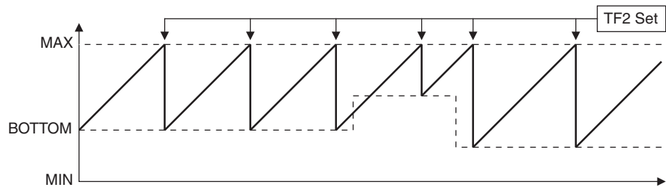
Figure 13-3. Timer 2 Waveform: Auto-Reload Mode (DCEN = 0)
