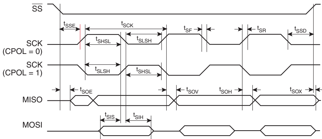
Figure 24-13. SPI Slave Timing (CPHA = 1)
