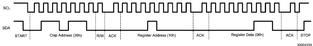
FIGURE 5. Write Sequence to the LM3509
