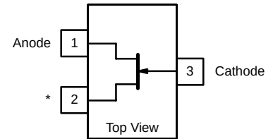
TO-236 (SOT-23)
