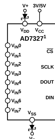
Figure 56. Schottky Diode Connection
