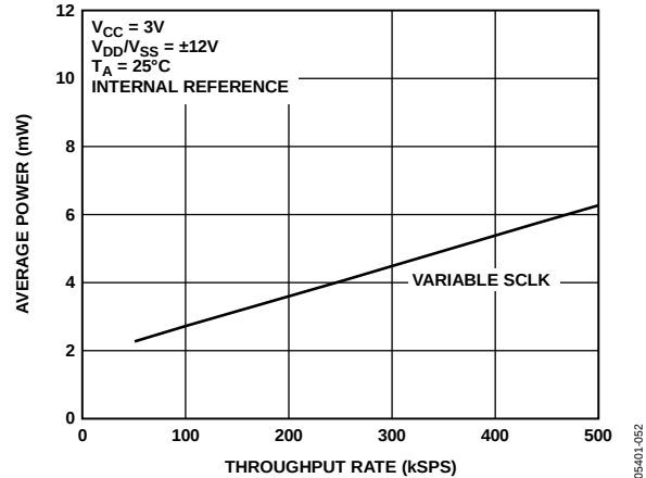
Figure 51. Power vs. Throughput Rate with 3 V V_{CC}
