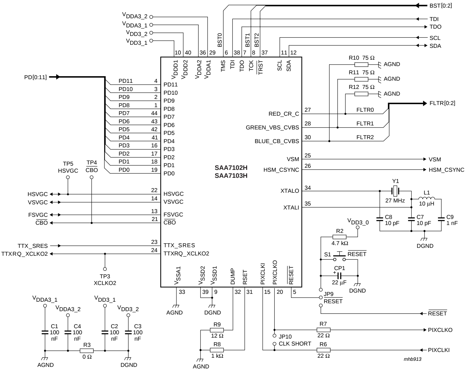
Fig 16. Application circuit
