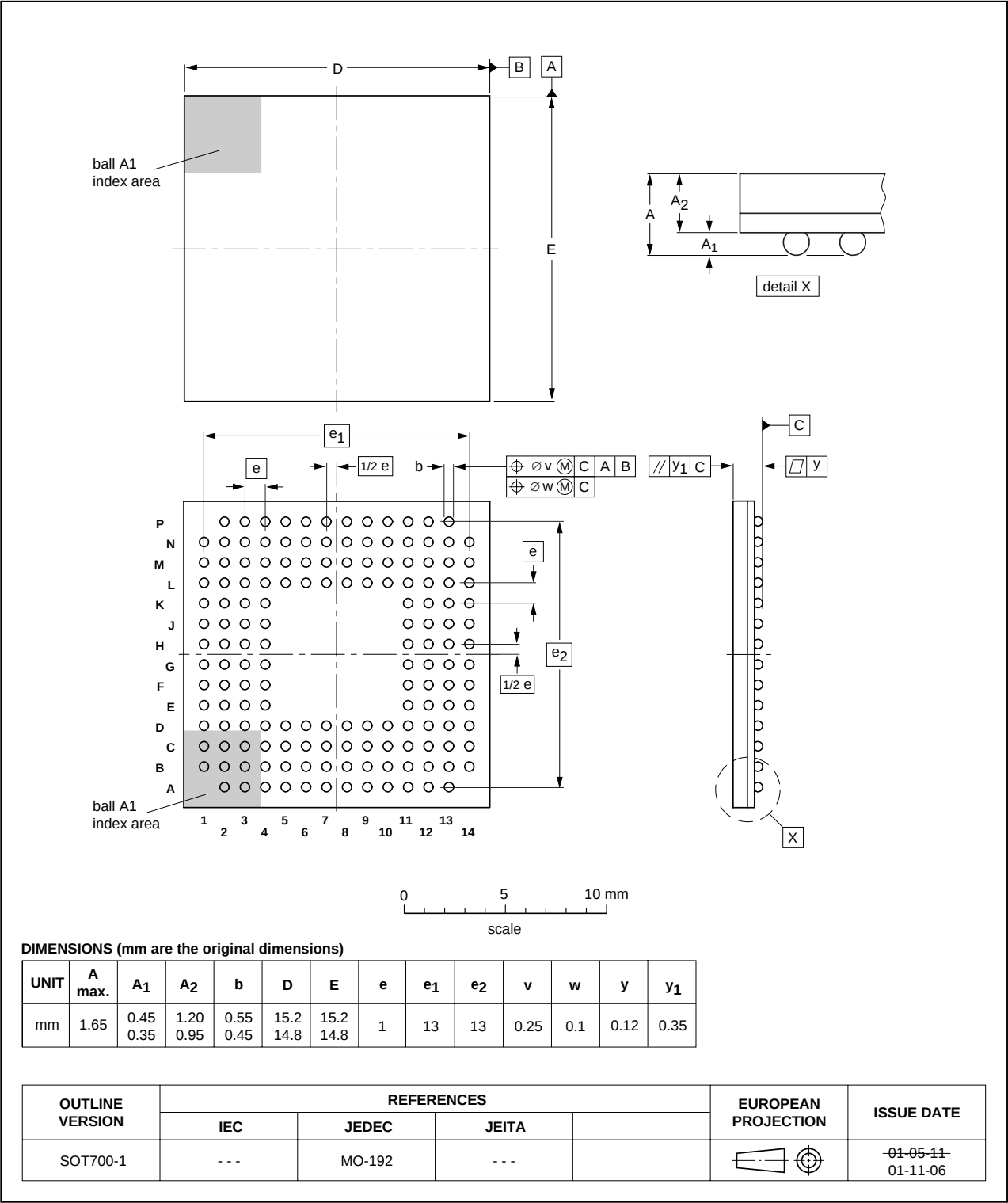
Fig 19. Package outline SOT700-1 (LBGA156)
