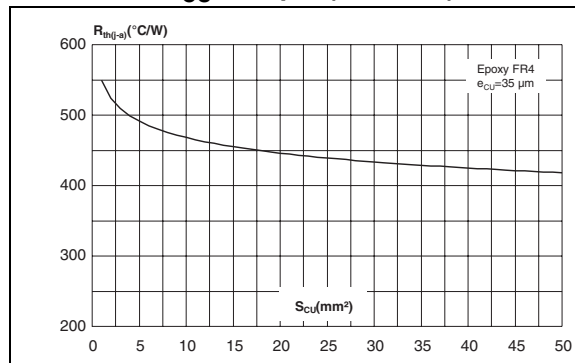
Figure 7. Thermal resistance junction to ambient versus copper surface under each lead - epoxy FR4 with recommended pad layout, e_{CU} = 35 \mu\text{m} (SOD-323)
