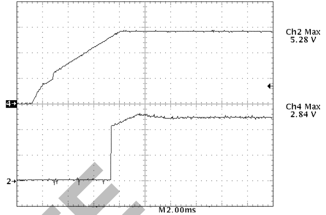
Figure 23. PWRGD Signal Becomes Logic High as V_{OUT} Enters -8.5\% of Lower PWRGD Threshold, V_{OUT} = +2.84 V (DAC = 10111)
