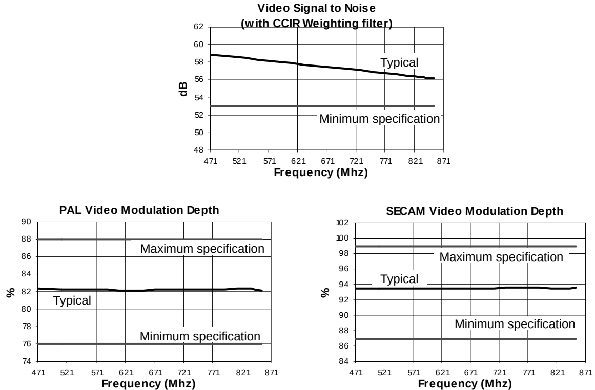
Figure 4. Typical Video Performance
