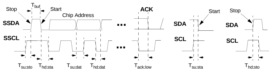
Figure 11. SSDA/SSCL Timing
