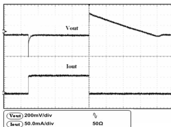
Figure 11. Load transient
