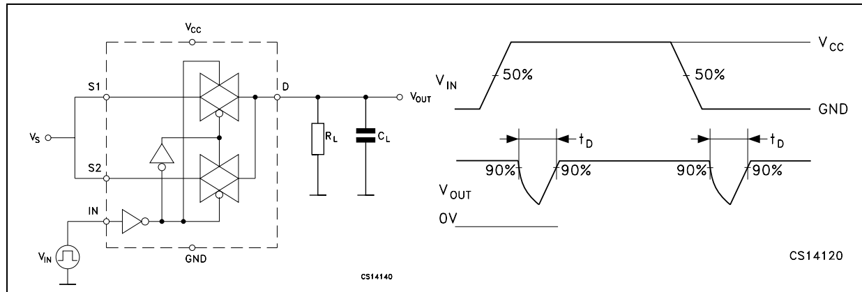
Figure 12. Switching time and charge injection ( V_{GEN} = 0 V, R_{GEN} = 0 \Omega , R_L = 1 M \Omega , C_L = 100 pF)
