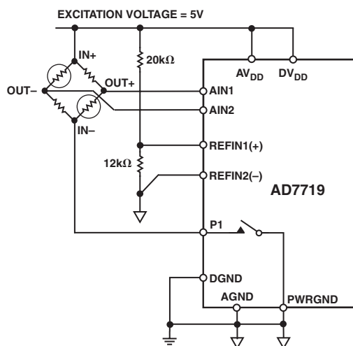
Figure 19. Pressure Measurement Using AD7719
